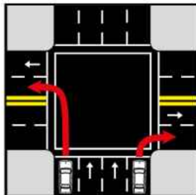
Turns from one-way to two-way
